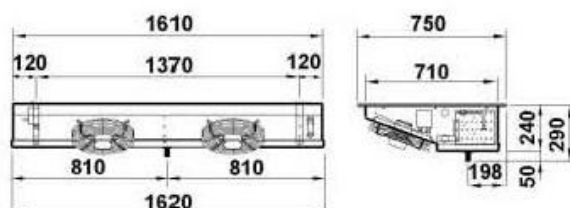
Evaporator GS340
